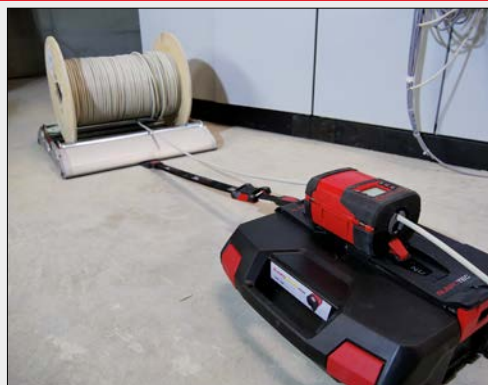
RUNPOMETER RM35 with connecting pad and belt fixed to cable drum roller PRO
