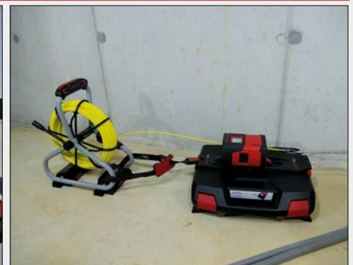
RM35 with Mounting plate- system case , Profi Set fiberglass rod Ø 4,5 mm
