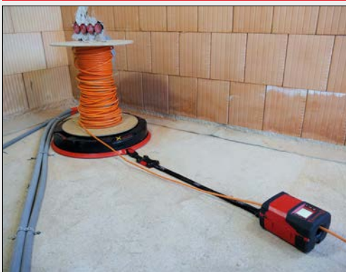
RUNPOMETER RM35 with belt and clip system connected to XB 500
